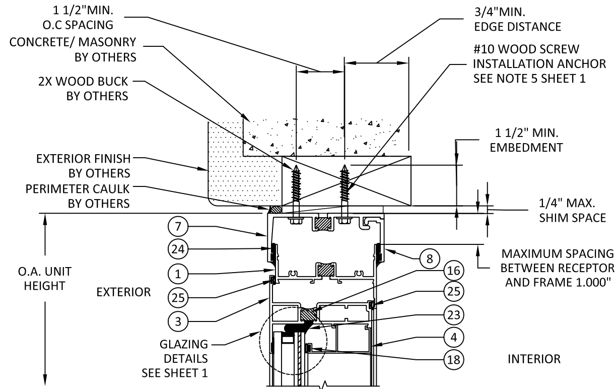
A 4 VERTICAL SECTION HEAD - 2X WOOD BUCK THROUGH FRAME INSTALLATION
