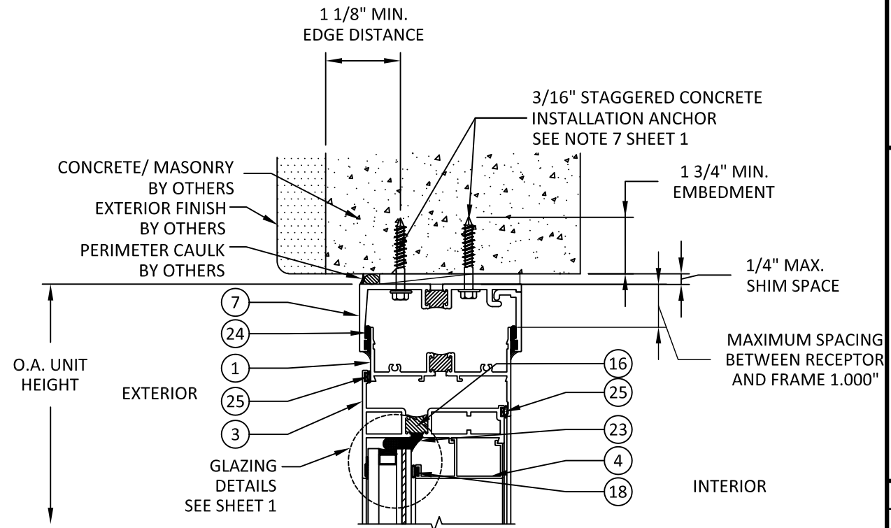
C 4 VERTICAL SECTION HEAD - CONCRETE OR CMU THROUGH FRAME INSTALLATION
