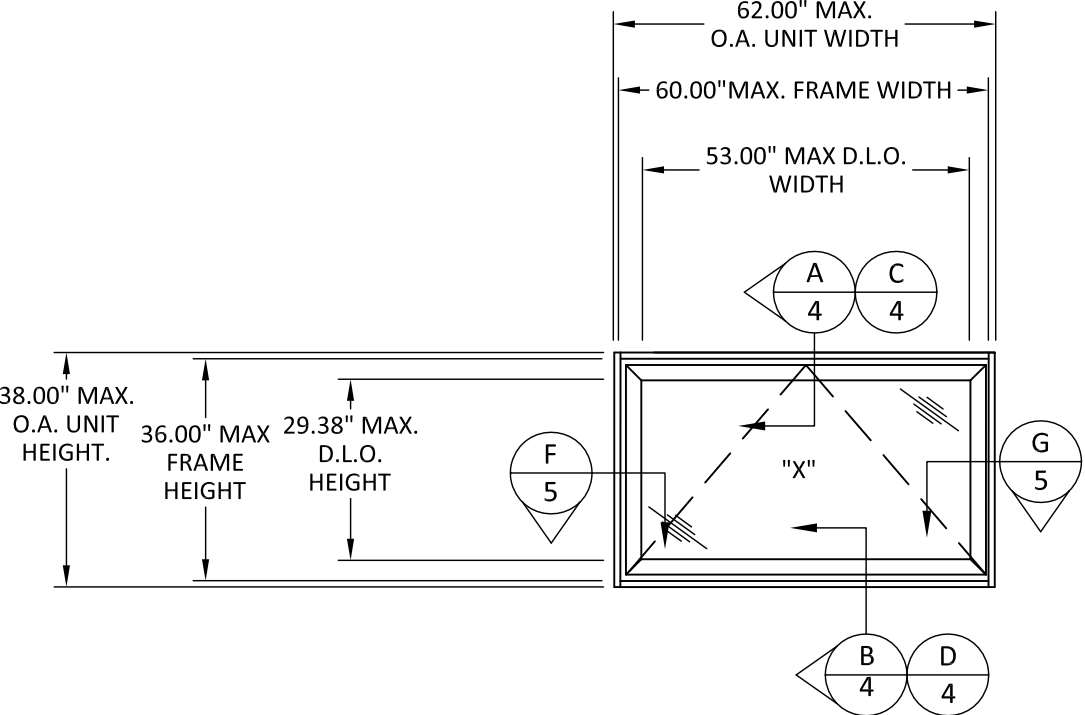
EXTERIOR ELEVATION PROJECT-OUT WINDOW
