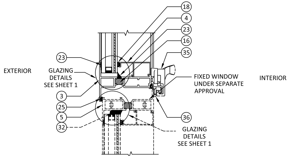
C 6 VERTICAL SECTION MEEETING RAIL PO/FX ( MAX SPAN 60")
