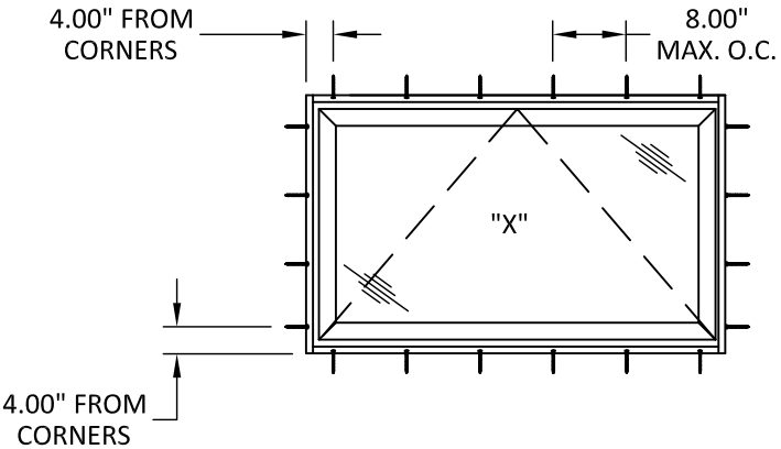
ANCHOR LAYOUT PROJECT-OUT WINDOW THROUGH FRAME INSTALLATION
