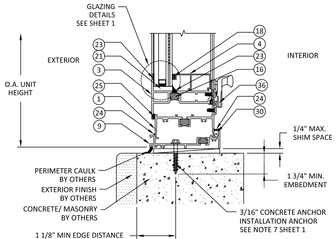
D 4 VERTICAL SECTION SILL - CONCRETE OR CMU THROUGH FRAME INSTALLATION
