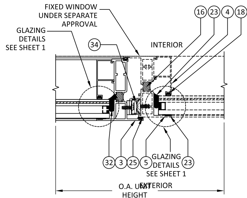
D HORIZONTAL SECTION 7 MEETING RAIL (MAX SPAN 60")
