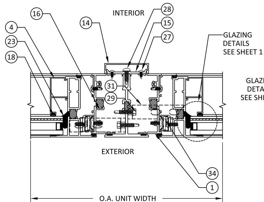
B HORIZONTAL SECTION 7 MULLION (SPAN UP TO 72")
