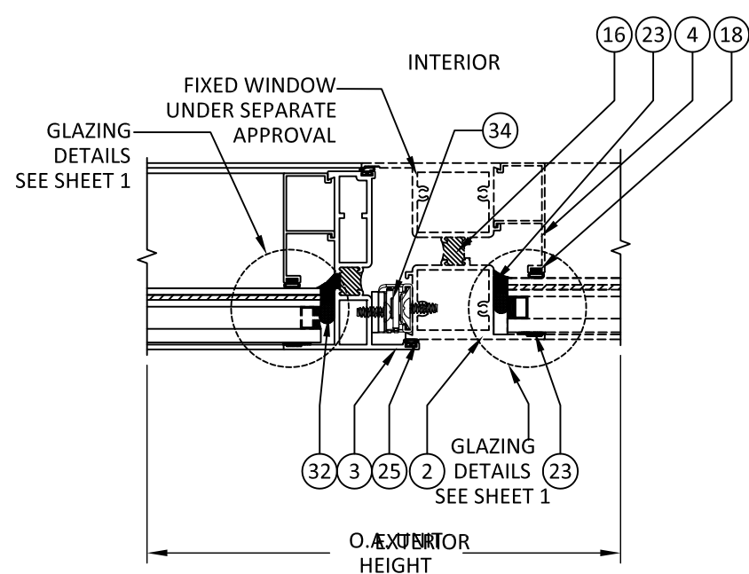
E HORIZONTAL SECTION 7 MEETING RAIL (MAX SPAN 72")
