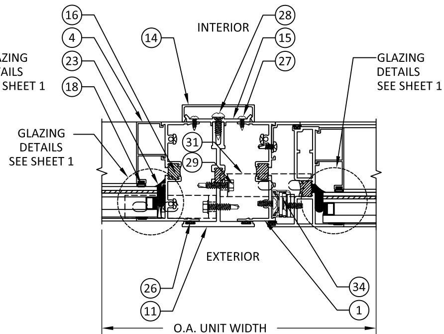
C HORIZONTAL SECTION 7 MULLION (SPAN UP TO 72")
