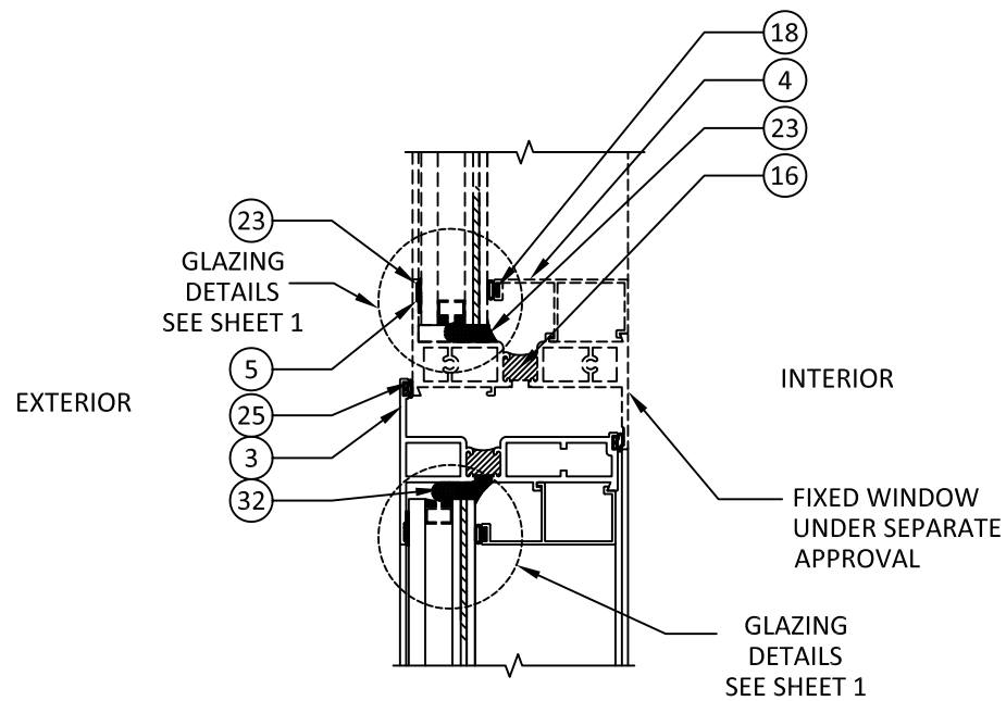
A 6 VERTICAL SECTION MEETING RAIL FX/PO( MAX SPAN 60")
