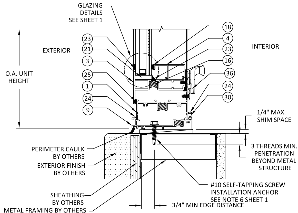
B 4 VERTICAL SECTION SILL - METAL STUD THROUGH FRAME INSTALLATION
