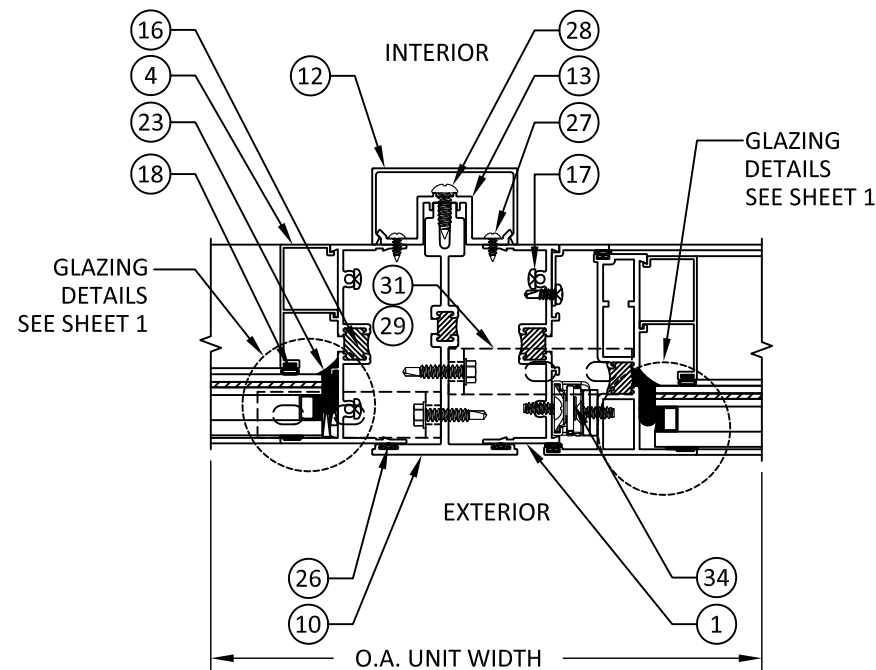
A HORIZONTAL SECTION 7 MULLION (SPAN LONGER THAN 72")
