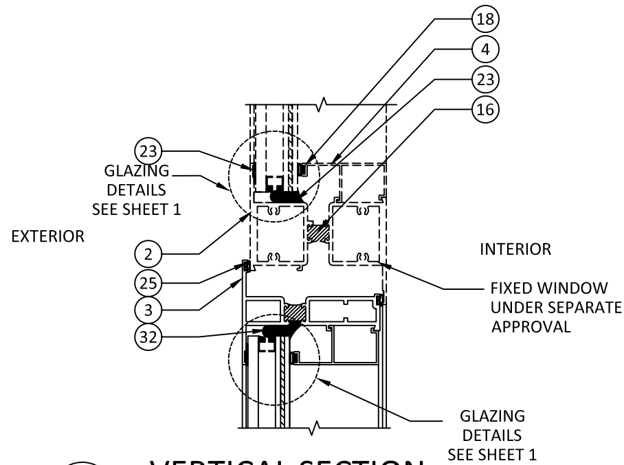
B 6 VERTICAL SECTION MEETING RAIL FX/PO ( MAX SPAN 72")
